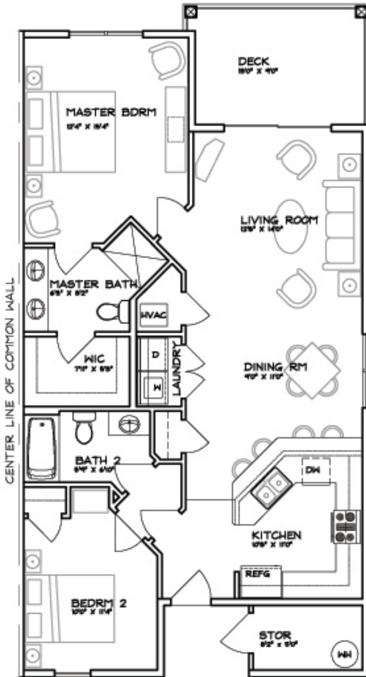
FLOOR PLAN EXTERIOR UNIT 1,022 SQ. FT.
